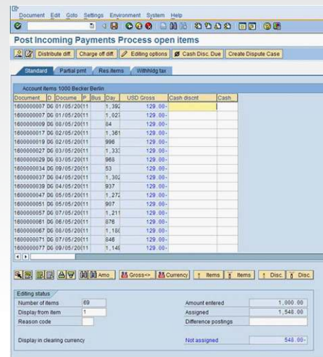
Figures 3 & 4: An incoming receivable statement in a spreadsheet (above) is automatically posted into the Incoming Cash SAP transaction (F-28).
